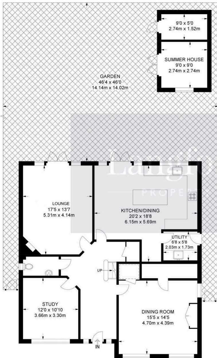
GROUND FLOOR 1208 SQ FT / 112.2 SQ M
